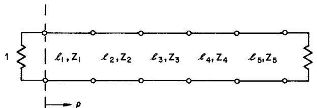
FIG. 1 5-SECTION TRANSMISSION-LINE LOWPASS FILTER WITH \ell_i = LENGTH OF i TH SECTION AND Z_i = CHARACTERISTIC IMPEDANCE OF i TH SECTION; \rho = REFLECTION COEFFICIENT.
